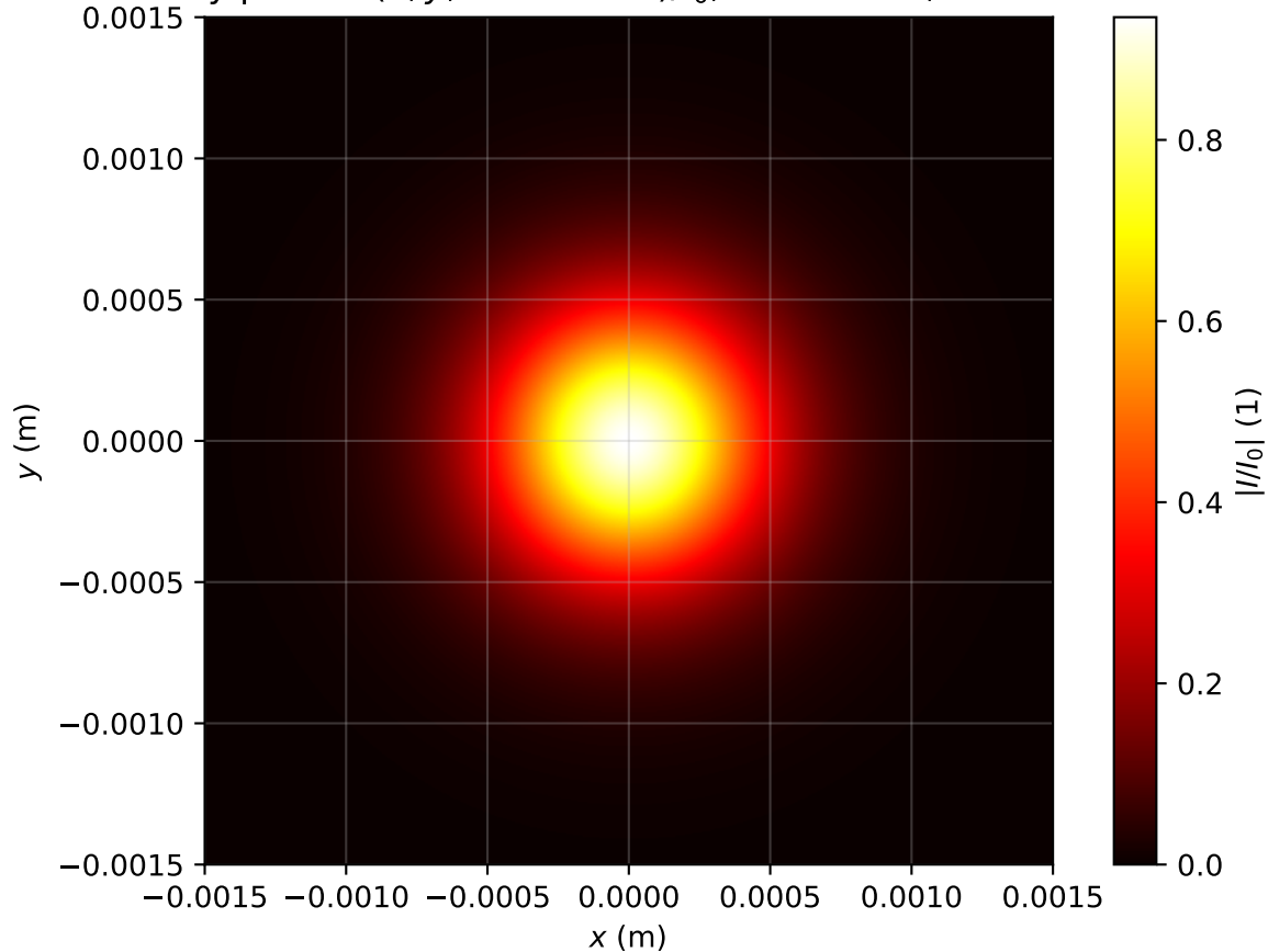
Intensity profile I(x, y, z = 1.592m)/I_0 , Pin=0.5Pcr, artificial time
